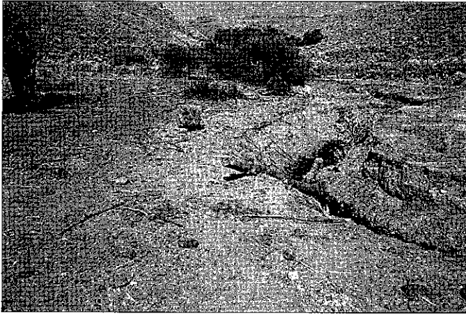
Season-long access by cattle damaged this long water gap. Water gaps should be only 3-6 m (10-20 ft) long and on straight stretches of streams with gentle banks. This area later improved after season of use was reduced from 4 months to 1 and stocking levels were decreased by 20%. The water gap will be eliminated when upland water sources are developed.
