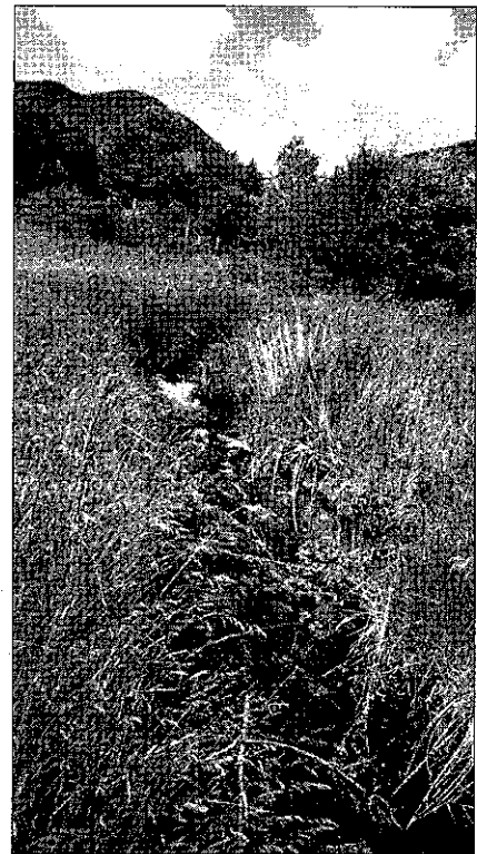
Herding livestock is effective for riparian habitat protection. Cattle graze this site a few weeks a year with herders daily moving them out of the riparian area to an upland site. When the vegetation shows a specified use level, grazing ceases.
